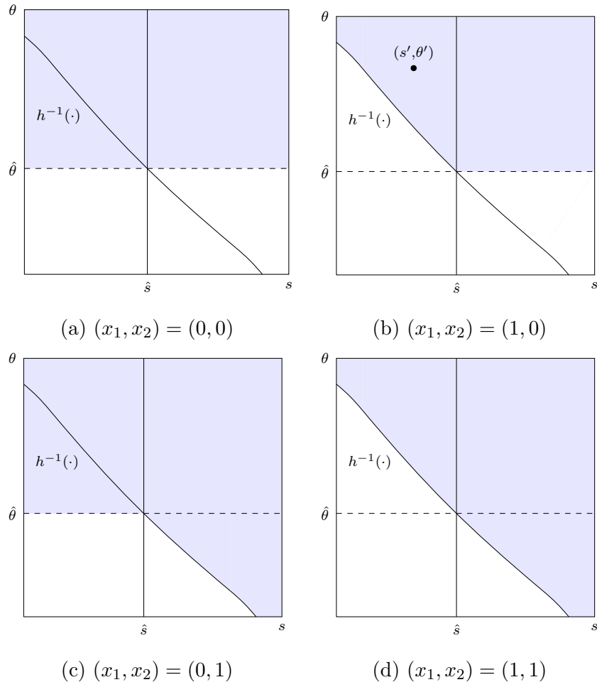
Figure 3: Decision Equivalence
